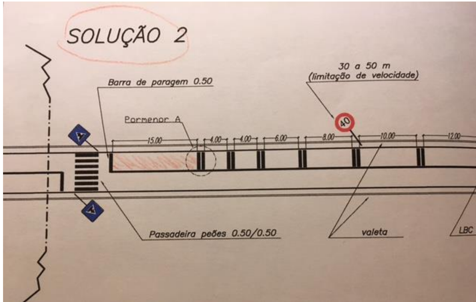
Scheme of disposition of the rumble strips
